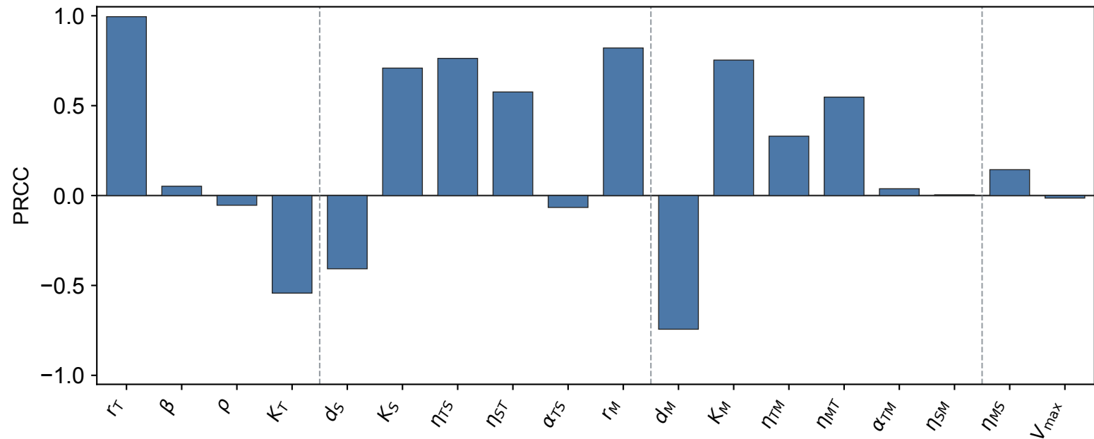
OVCAR4: PRCC on AUC of Total cancer-associated burden T(t) + S(t) + M(t) | Tumor+MSC+M2
